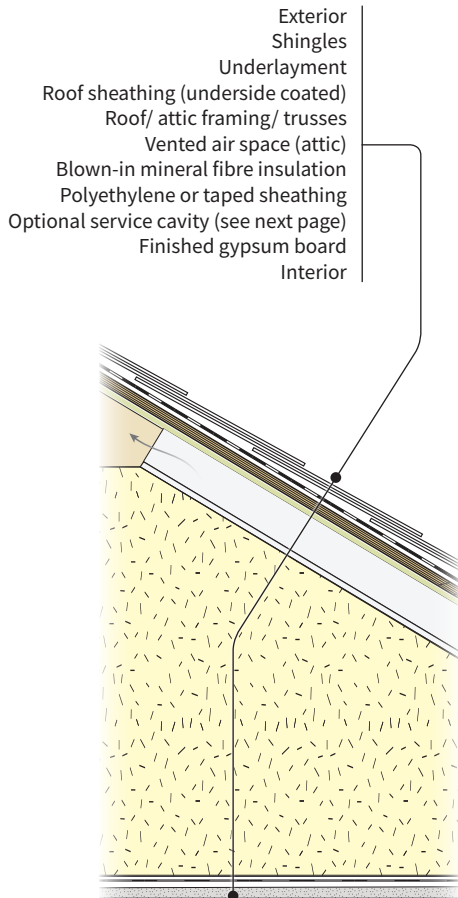
Section view of interior insulated vented attic roof
